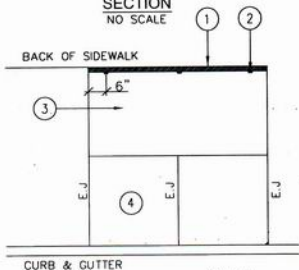
PLAN NO SCALE
