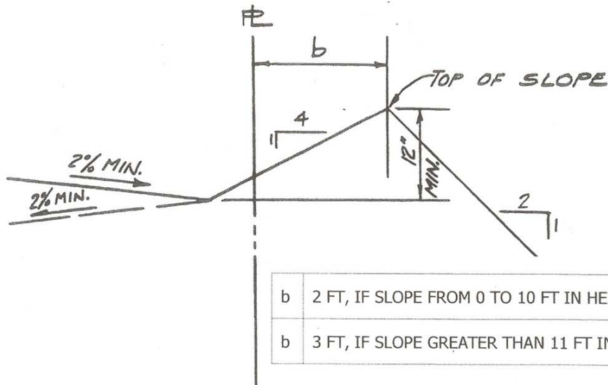
BERM DETAIL (SEE STANDARD DETAIL NO. 328)
