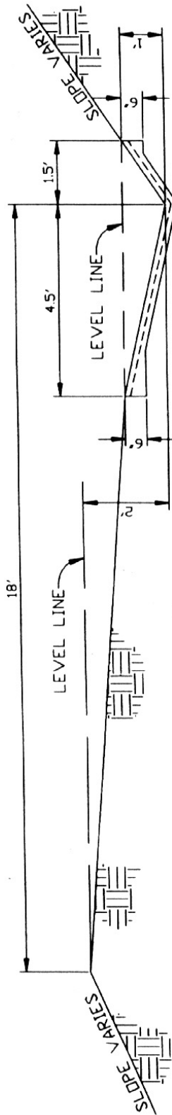
18' TERRACE DRAIN
